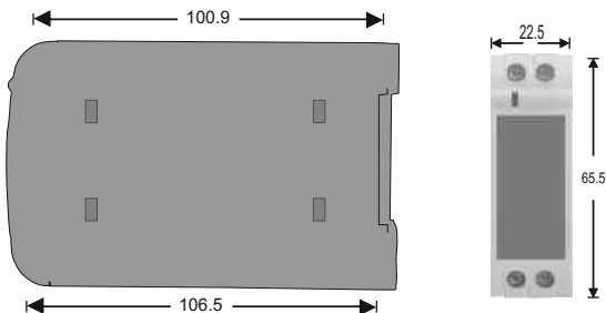
Fig. 7. Side View & Front view
